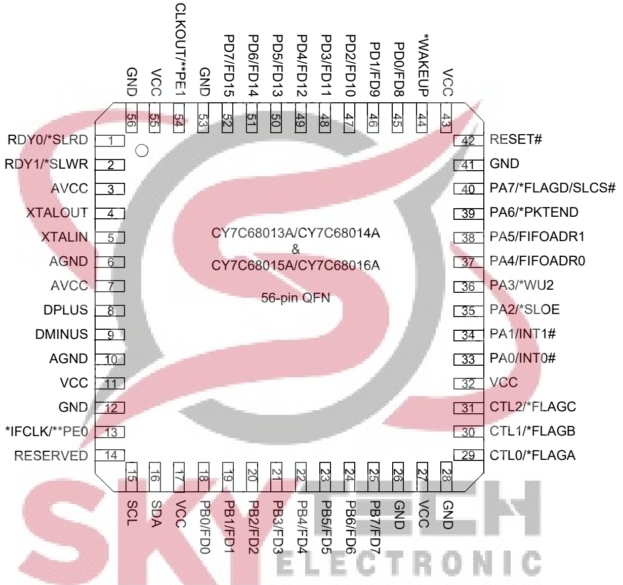
Figure 10. CY7C68013A/14A/15A/16A 56-Pin QFN Pin Assignment
